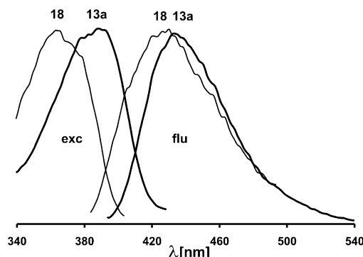
Figure 1. Excitation and emission spectra of 4-cyano- vs. 4-trifluoromethylcarbostyrils 13a and 18 in water.
